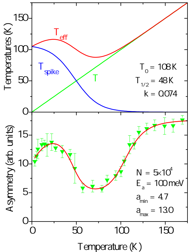
FIG. 4: Simulation of the total asymmetry in the \text{Si}_{0.09}\text{Ge}_{0.91} experiment of Ref. 22 (Fig. 3). Top: The effective temperature at the muon site is a sum of the lattice temperature, T , and a local, temperature-like effect T_{spike} : T_{eff} = T_{spike} + T . The spike temperature is given by Eq. 1 with the parameters shown in the insert. Bottom: Total asymmetry obtained from Fig. 3. The red line is a simulation of the asymmetry using a total fraction as described in Eq. 2 with the effective temperature T_{eff} shown in the upper frame. The corresponding parameters describing the thermal recovery above 100 K are shown in the insert.
