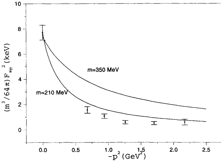
Fig. 2. Transition form factor for the anomalous process \pi^0 \rightarrow \gamma^* \gamma in the space-like region as calculated in the renormalized version with different constituent quark masses. The data are from Ref. [25].
