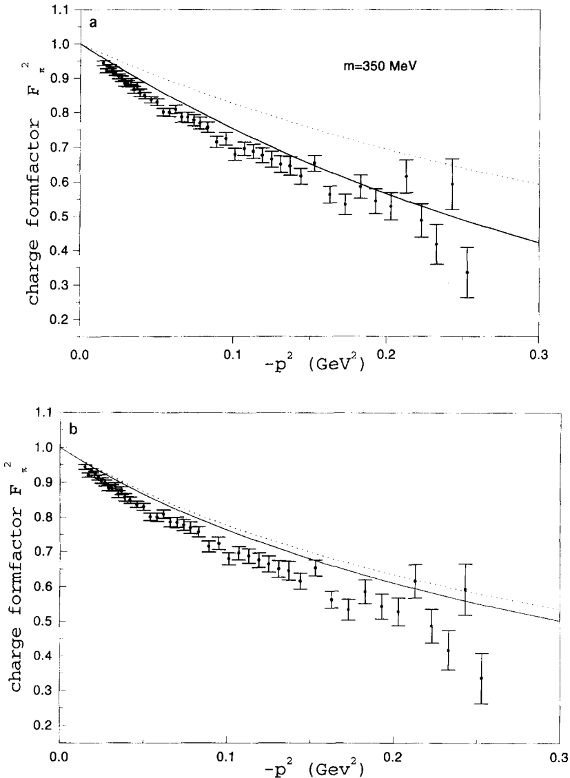
Fig. 1. Pion form factor in the space-like region. The results of the renormalized (solid) and regularized (dashed) models for small and large constituent quark masses are compared to experimental data [21].
