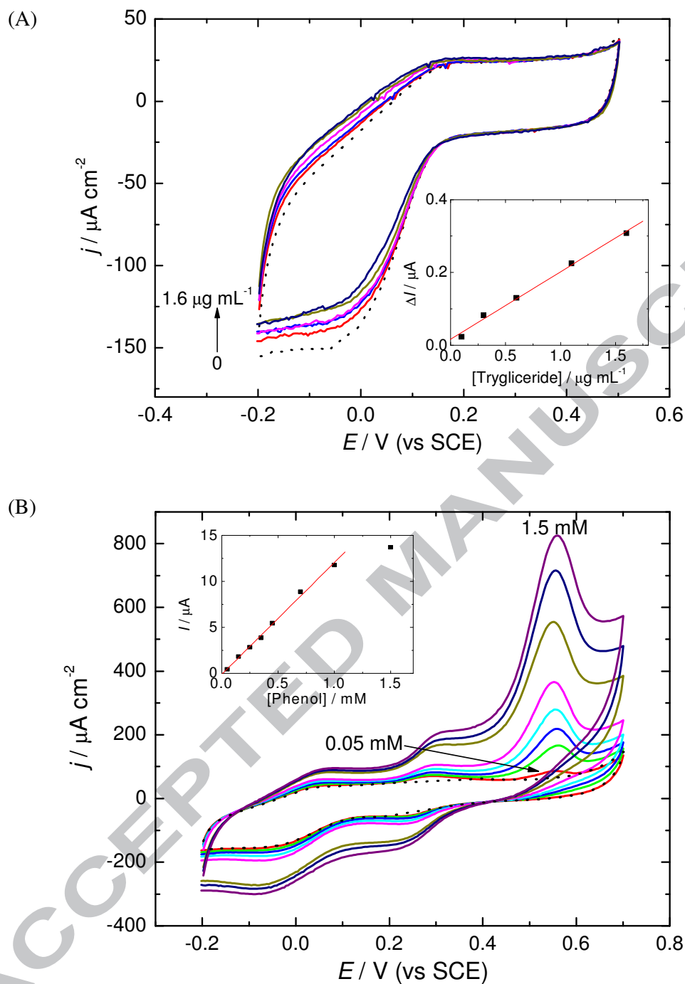
Fig. 4. Cyclic voltammograms at GC/MWCNT- BmimNTF 2 /Lip in 0.1 M PB, pH 7.0 after addition of glyceryl tributyrate of ( \mu\text{g mL}^{-1} ): 0; 0.1; 0.3; 0.6; 1.1; 1.6 (A) and phenol of (mM): 0; 0.05; 0.15; 0.25; 0.35; 0.45; 0.7; 1.0; 1.5 (B) dissolved in BmimNO 3 . Scan rate 10 \text{ mV s}^{-1} .
